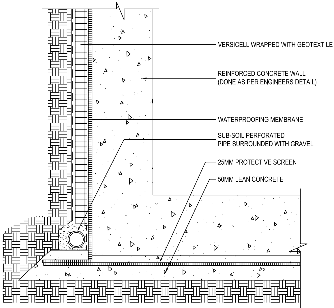
RETAINING WALL SECTIONAL DETAIL
