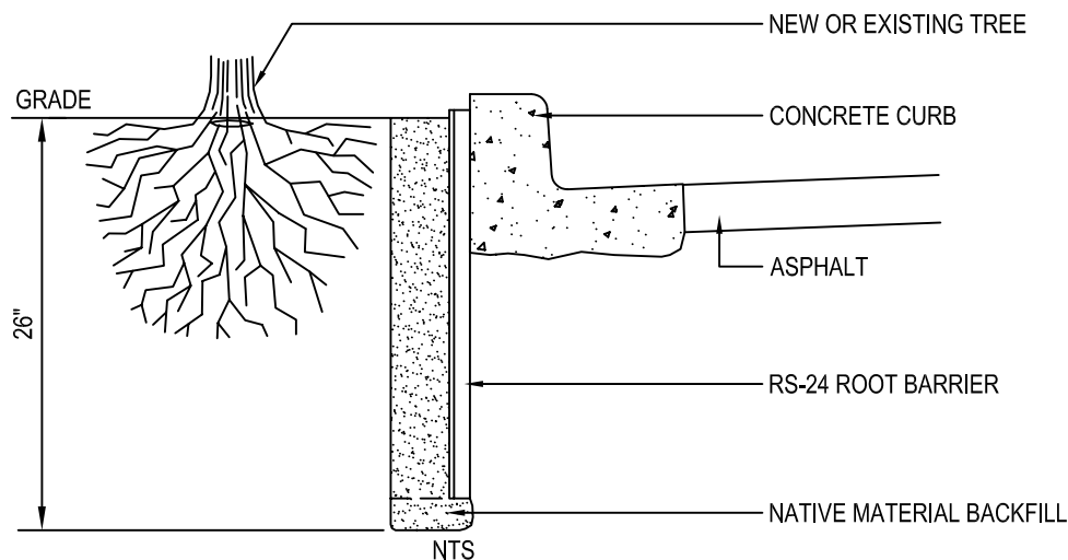
SECTION
